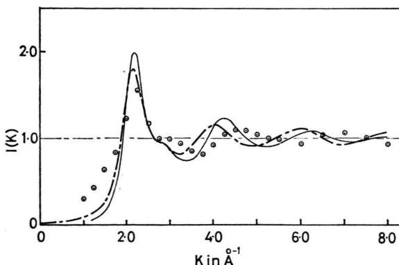
Fig. 1. Interference functions. — I_{\text{Sb}}(K) at 660 °C by Waseda and Suzuki 7 . --- I_{\text{T}}(K) , \sigma_{\text{A}}=3.11 Å, \sigma_{\text{B}}=2.33 Å, \eta=0.41 , c_{\text{A}}=0.60 . \odot points read from the published graph of I_{\text{Sb}}(K) by Knoll and Steeb 8 .
